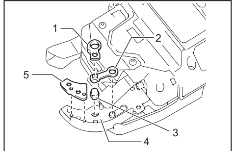
► 1. Cutter B 2. Link arm A 3. Cutter A 4. Arm plate A 5. Top plate
