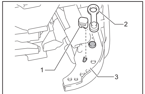
► 1. Cutter A 2. Link arm A 3. Arm plate A
